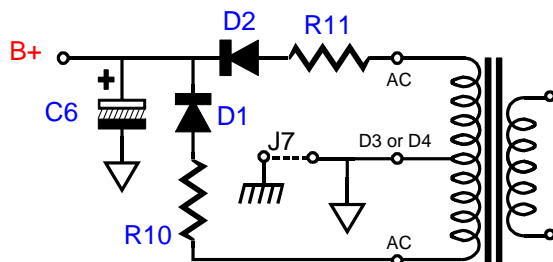
Center-Tapped Transformer
